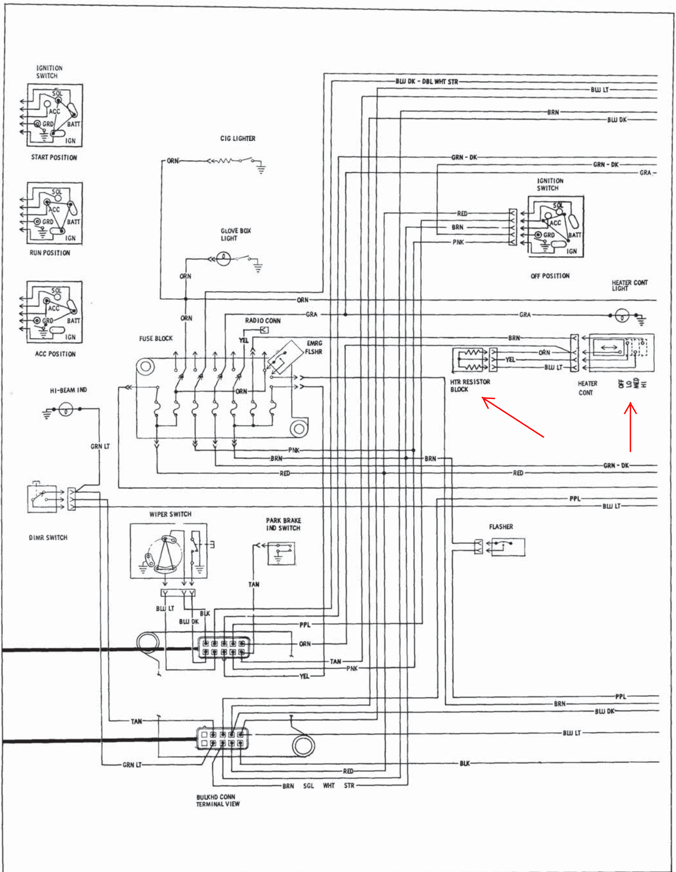
Fig. 12-2 Instrument Panel Harness
