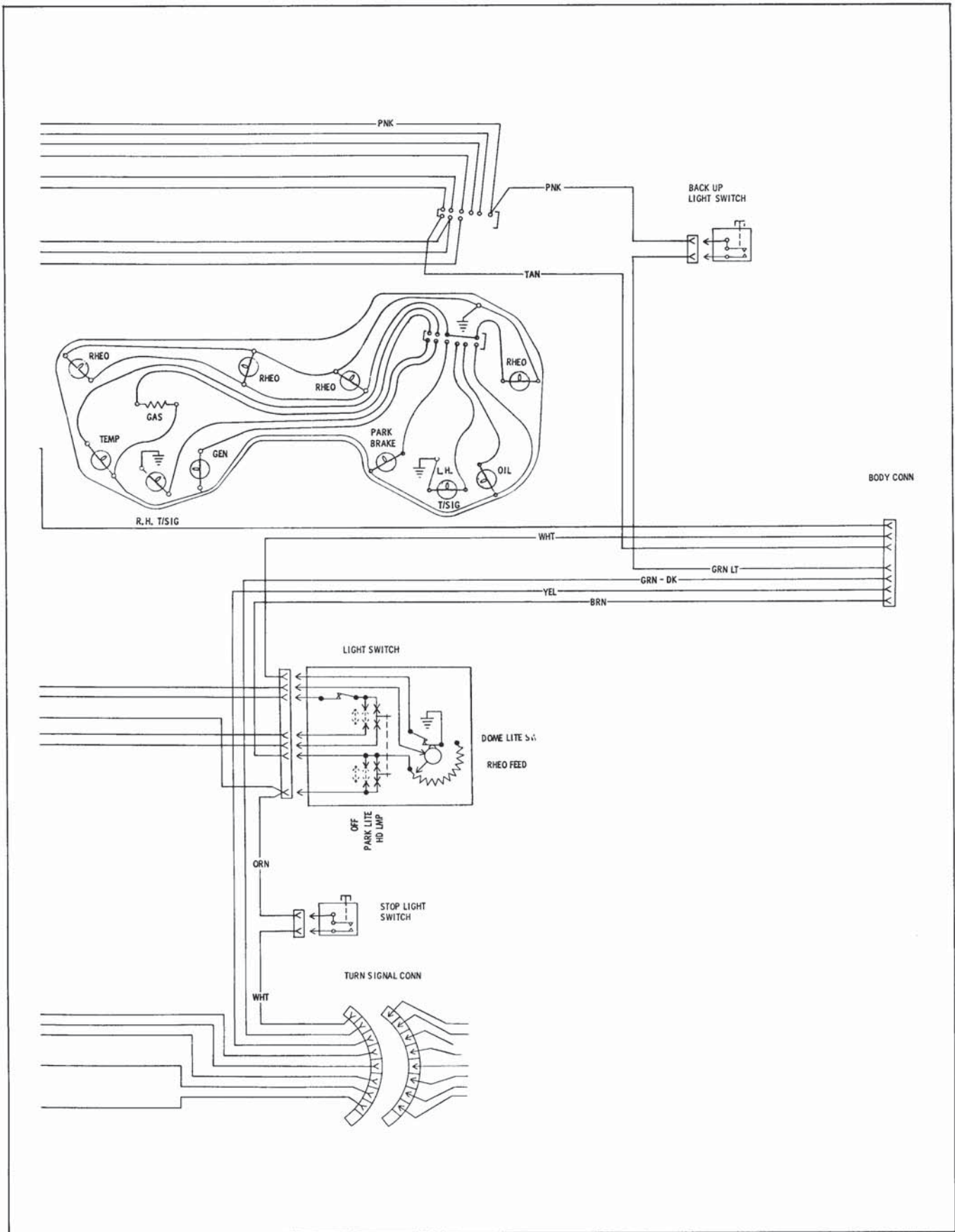
Fig. 12-2A Instrument Panel Harness - Continued
