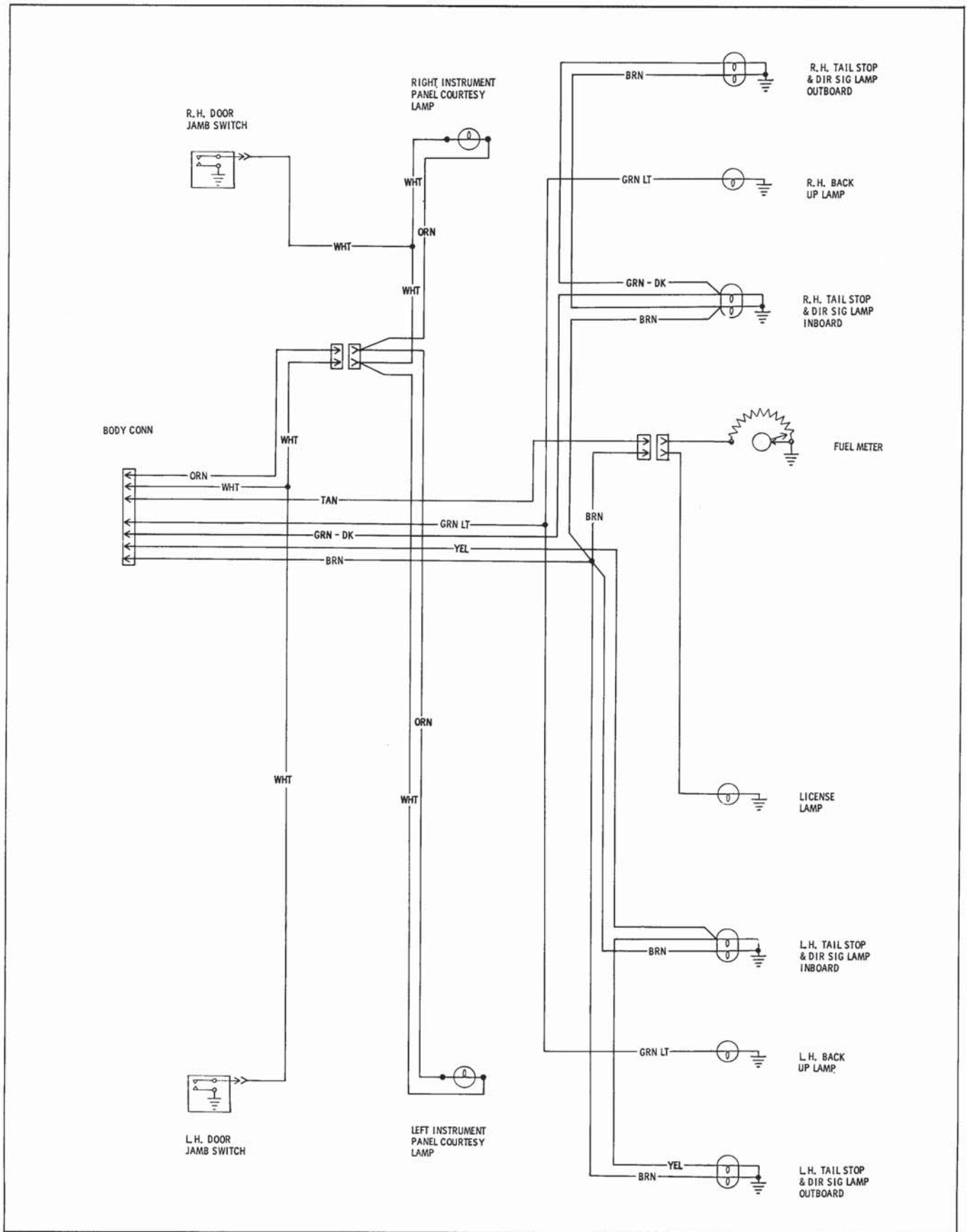
Fig. 12-3 Rear End Harness
