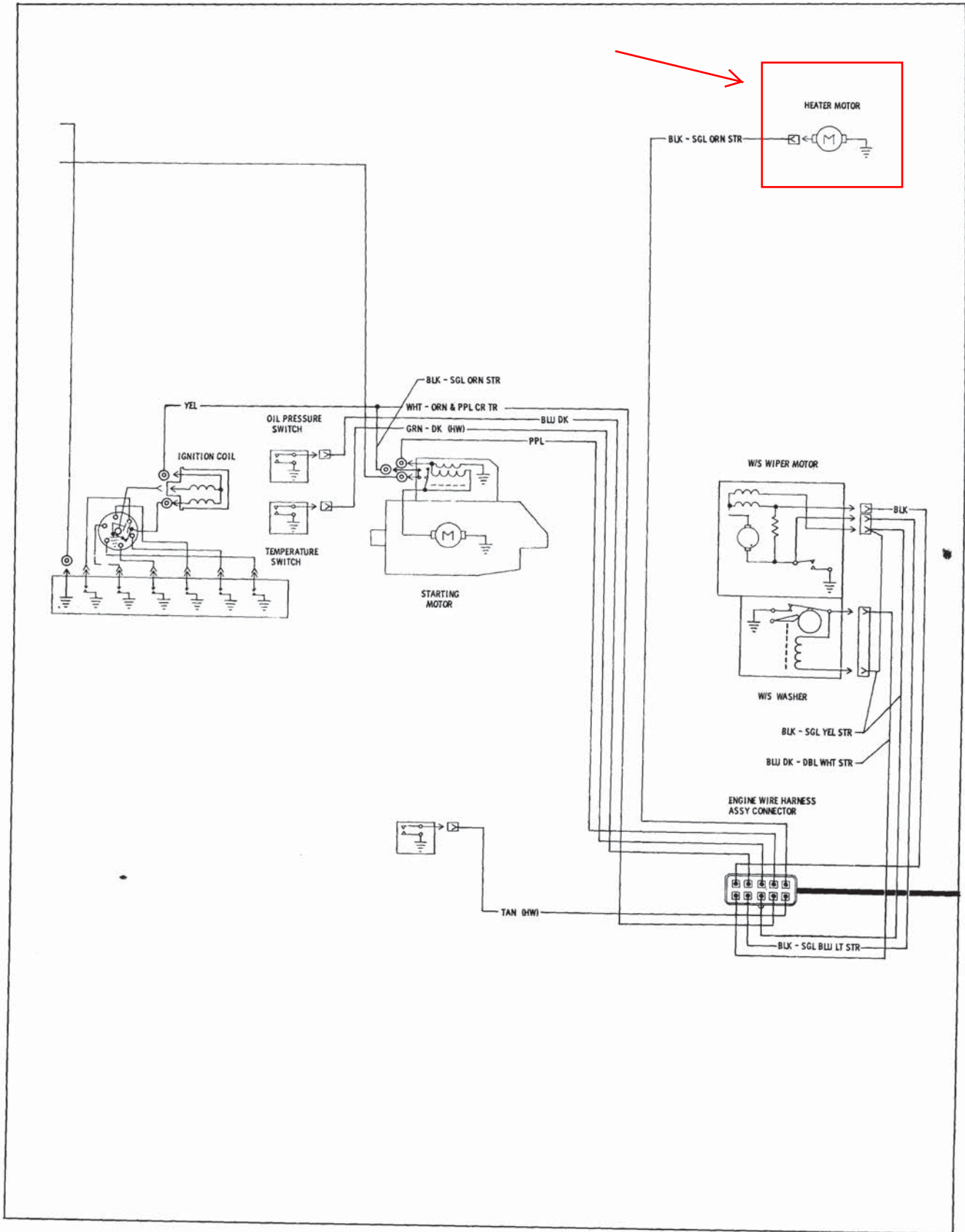
Fig. 12-1A 6 Cyl. Engine Harness
