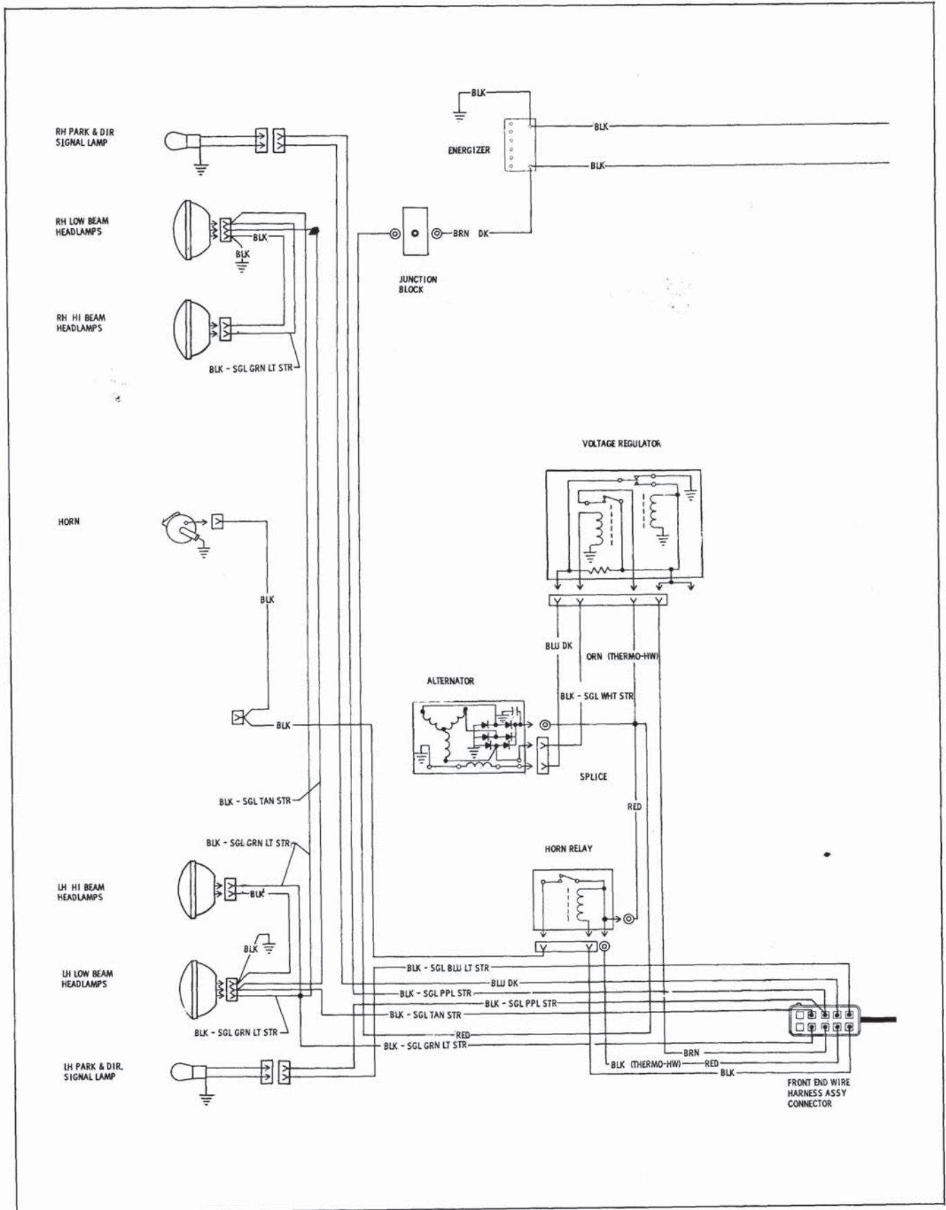
Fig. 12-1 Forward Lamp Harness
